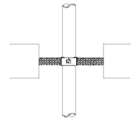
Cast-into Mineral Wool Boards
